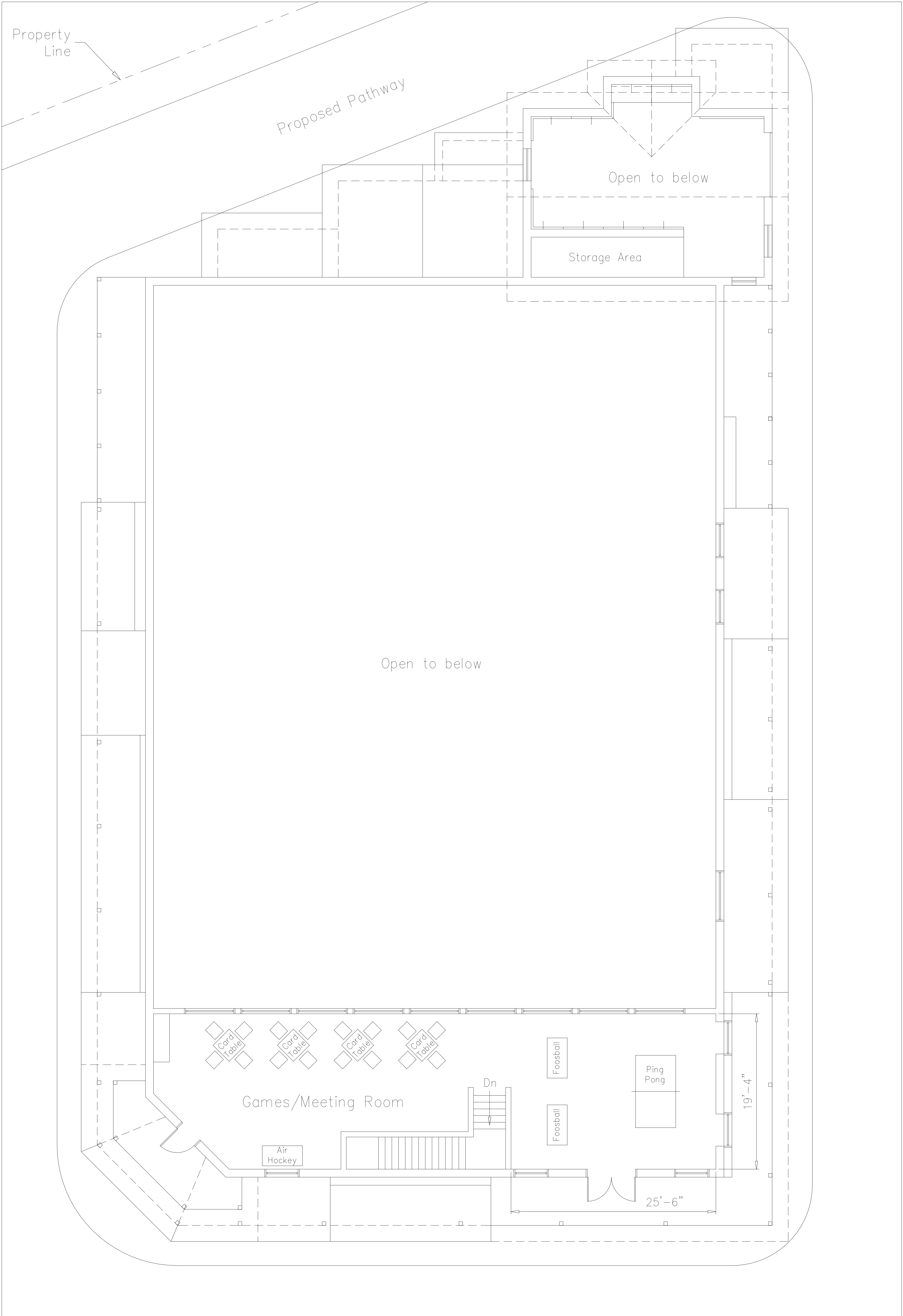
Timberline Ranch Proposed Activity Centre Preliminary Upper Floor Plan
