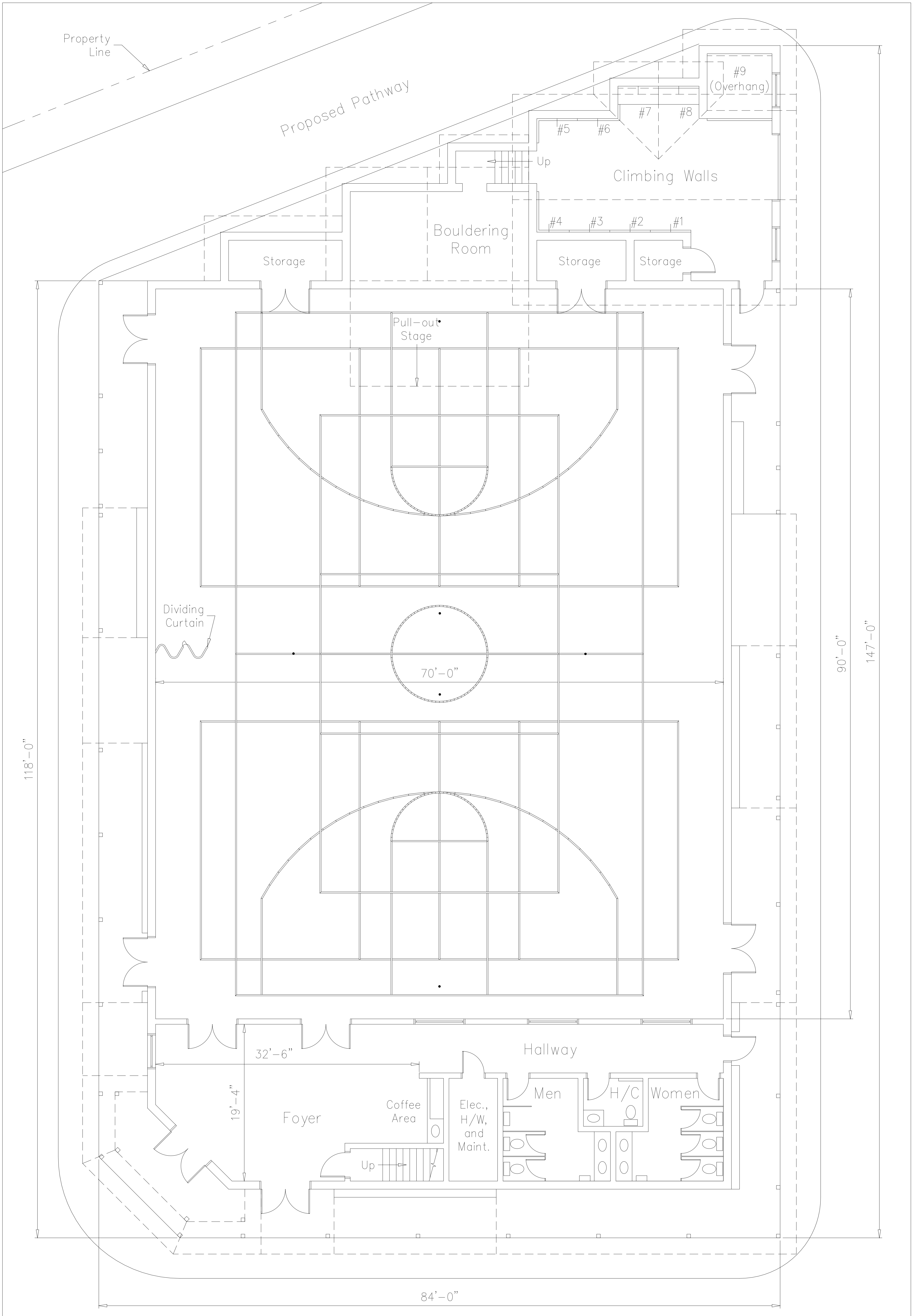
Timberline Ranch Proposed Activity Centre Preliminary Main Floor Plan
